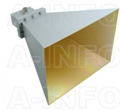
LB-510-15-C-7/16F Standard Gain Horn Antenna 1.45-2.2GHz 15dB Gain 7/16(DIN) Female
