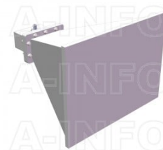
LB-510-15-C-NFSPO Standard Gain Horn Antenna 1.45-2.2GHz 15dB Gain N Type Female
