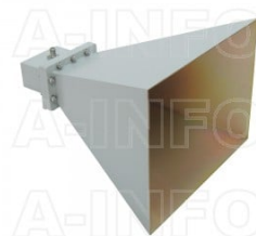
LB-510-15-C-NF Standard Gain Horn Antenna 1.45-2.2GHz 15dB Gain N Type Female
