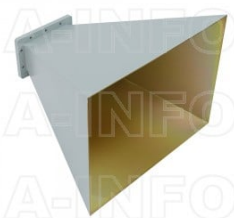
LB-510-15-A Standard Gain Horn Antenna 1.45-2.2GHz 15dB Gain Rectangular Waveguide Interface
